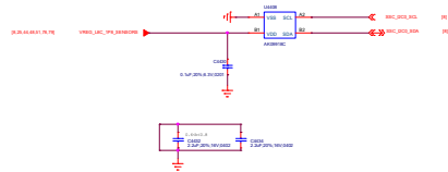
Magnetic Sensor
