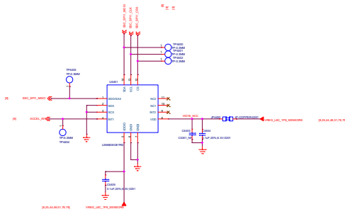
Magnetic Sensor
